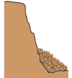
Eventually after repeated freezing and thawing, the rock breaks off.
